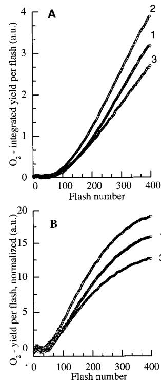
FIGURE 2: Kinetics of photoactivation of apo-WOC-PSII membranes with flashes of increasing flash duration. (A) Curve 1, without added bicarbonate; curve 2, after addition of 25 \mu\text{M} \text{NaHCO}_3 ; curve 3, after addition of 4 mM \text{NaHCO}_3 . (B) Normalized \text{O}_2 yield per unit flash length from panel A (normalized by dividing by the light pulse duration of each flash). Assay conditions are same as in Figure 1 except the concentration of \text{MnCl}_2 was 2 \mu\text{M} (2 Mn/PSII).
